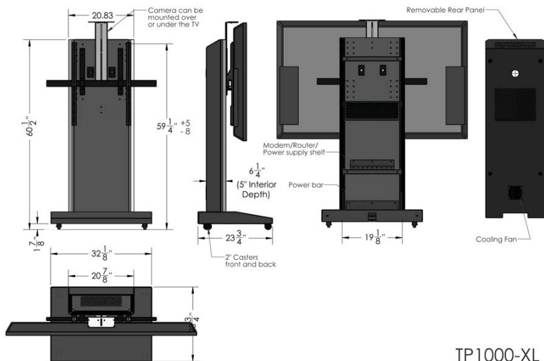
TP1000-XL
